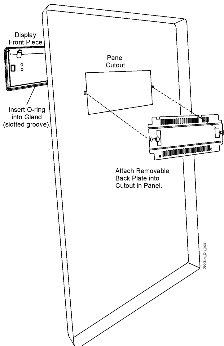
Figure 4: Attaching the display into panel cutout
