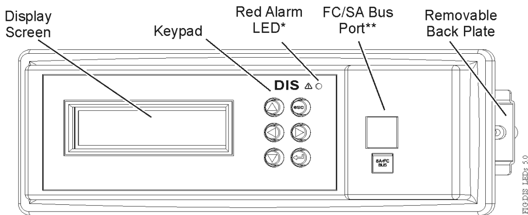
Figure 2: FX-DIS1710 physical features
