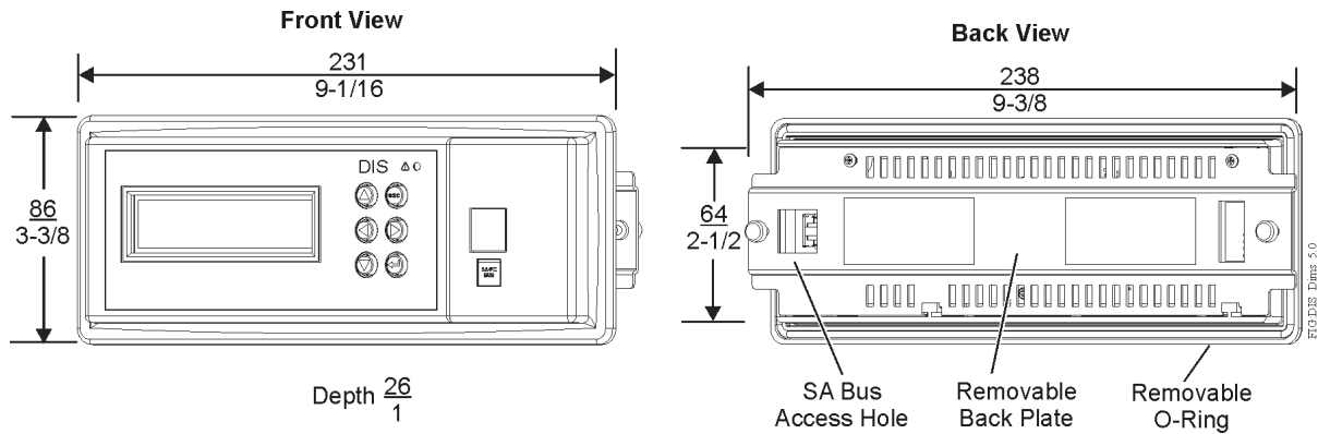
Figure 1: FX-DIS1710 Mounting Dimensions, mm/in.
