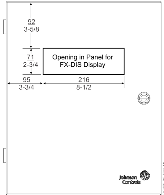
Figure 3: FX-DIS1710 Panel Cutout Dimensions, mm/in.
