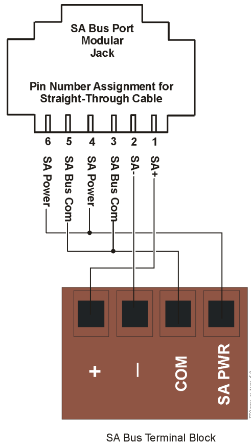
Figure 7: Wiring cable to SA bus terminal block
