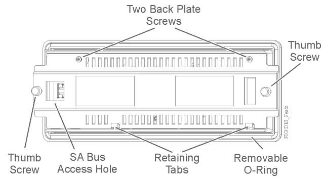
Figure 5: FX-DIS1710 back plate
