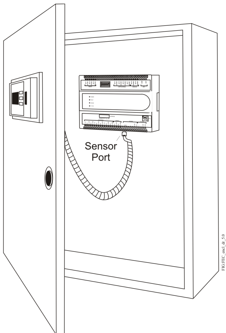
Figure 6: Connecting the SA bus cable
